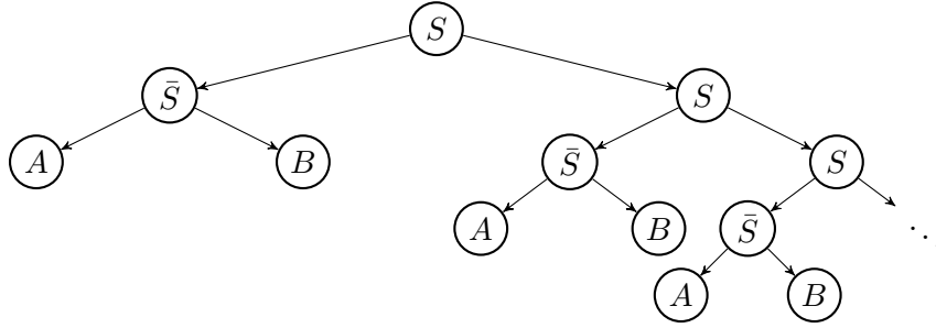
Figure 7.0.1: Graphical representation of _G \Delta w
