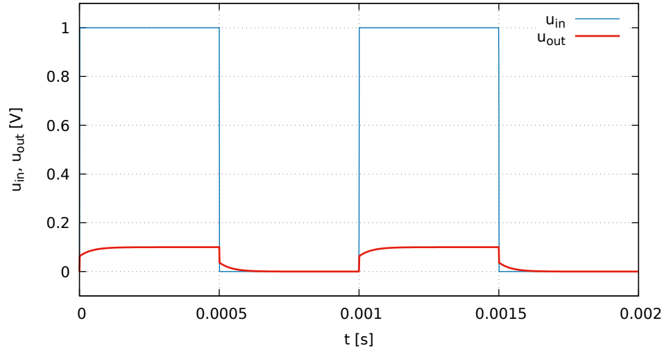
Uncompensated divider 1:10 (smaller Cx)
