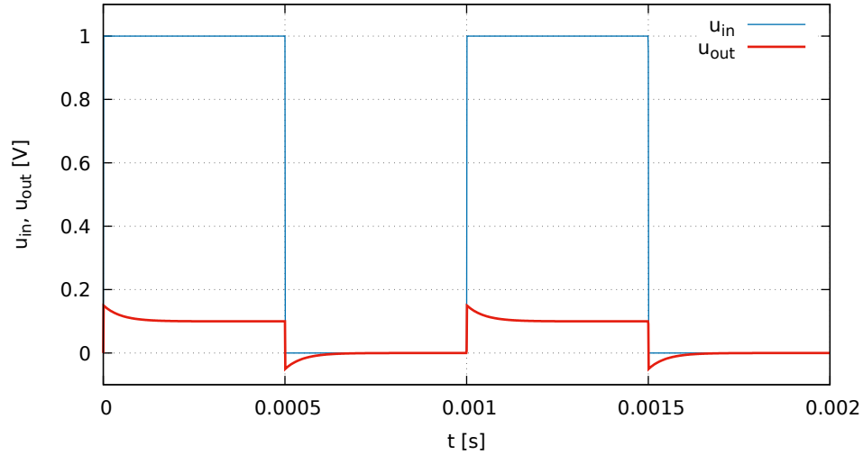
Uncompensated divider 1:10 (larger Cx)
