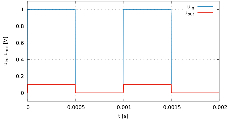
Frequency compensated divider 1:10
