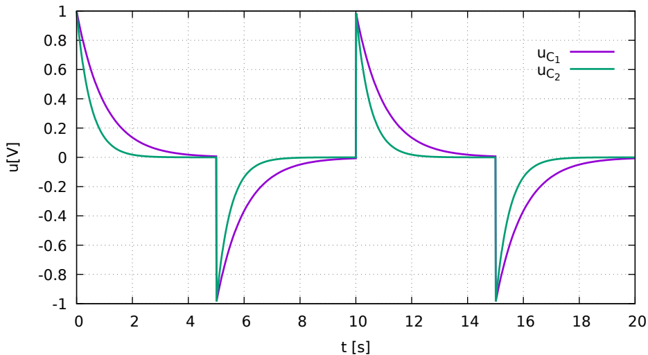
RC Circuit Pulse Response ( U_{\text{step}}=1\text{V} , R_1=1\Omega , R_2=0.5\Omega , C_1=C_2=1\text{F} )
