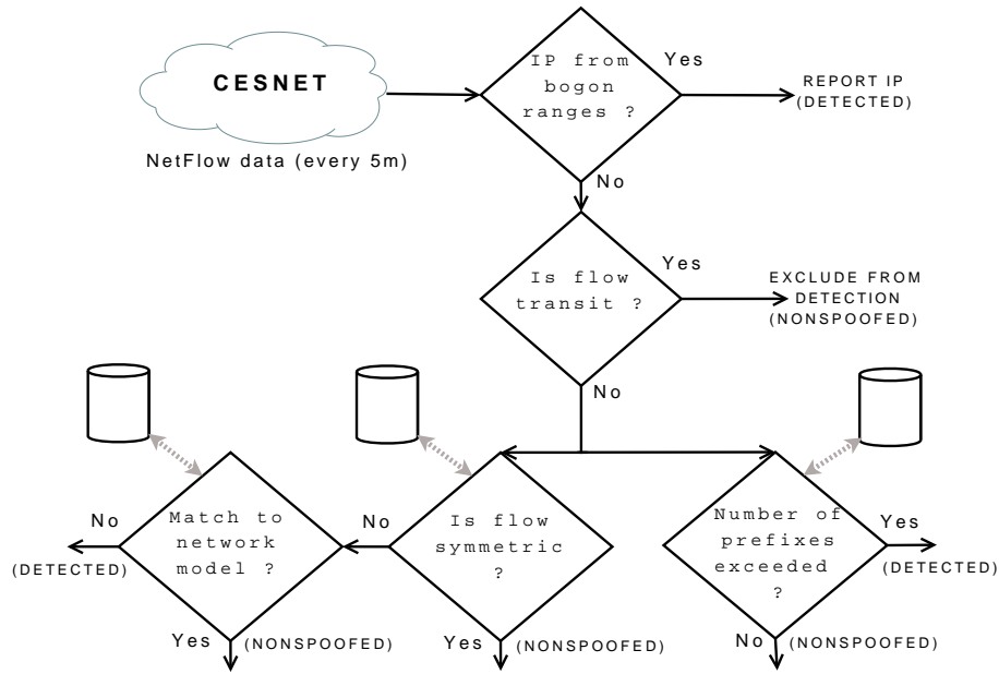
Fig. 1. Algorithm scheme.
