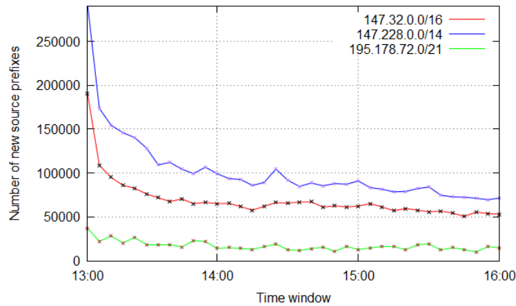
Fig. 7. Number of source prefixes reported per destination prefix by the model of new source prefixes.
