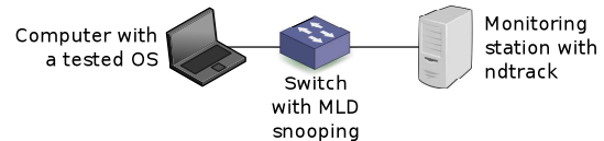
Figure 4: Network topology for experiments with network with active MLD snooping.
