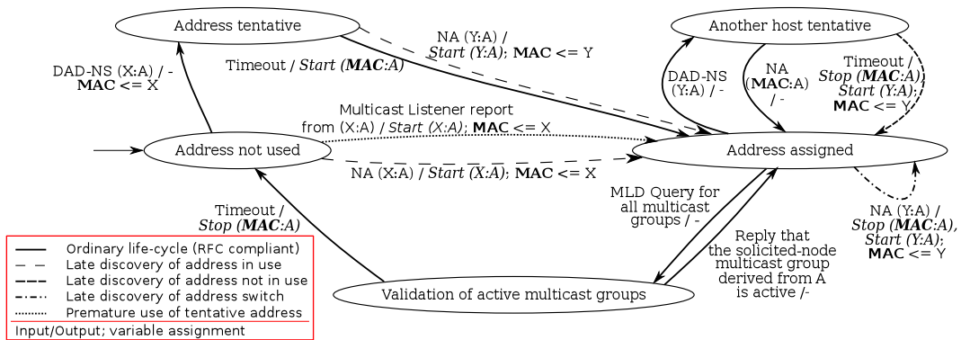
Figure 1: The life-cycle of an IPv6 address A can be monitored by the Mealy FSM extended by the variable MAC to store the MAC address of the interface that currently uses A. Binding between MAC address X and A is denoted as (X:A).
