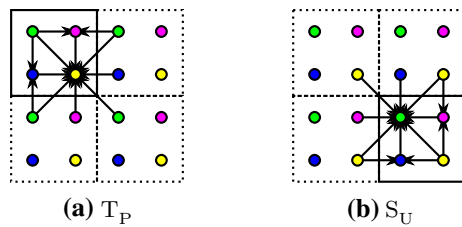
Fig. 11 2-D dataflow diagram, CDF 5/3 wavelet, Monolithic scheme. The solid box corresponds to the output coefficients
