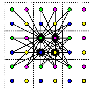
Fig. 5 2-D dataflow diagram, CDF 5/3 wavelet, Polyphase scheme. The solid box in the middle corresponds to the output coefficients
