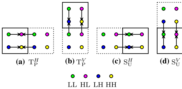
Fig. 3 2-D dataflow diagram, CDF 5/3 wavelet, Sweldens lifting scheme. The displayed part of the calculation results in the coefficients inside of the solid box . The dotted boxes refer to the surrounding threads
