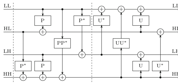
Fig. 10 Block diagram of the Monolithic scheme. The dashed vertical lines indicate barriers. The left half corresponds to the predict operator, whereas the right half to the update
