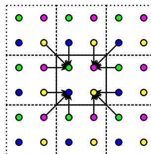
Fig. 16 2-D dataflow diagram, CDF 5/3 wavelet, Polyphase* scheme. The solid box corresponds to the output
