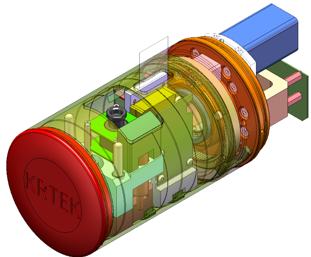
Fig. 1. Construction detail of sensoric head.
