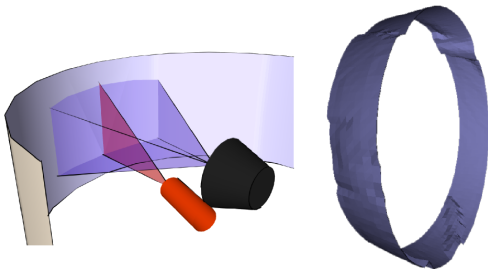
Fig. 3. Elevation profile reconstruction.
